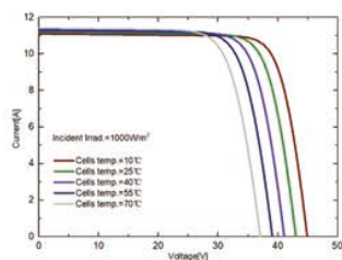
I-V Curves of HNG375QHES at different cell temperature
