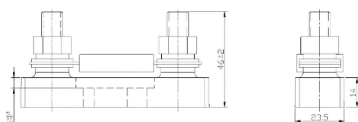
MEGA fuse
