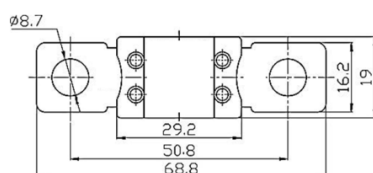
MEGA fuse
