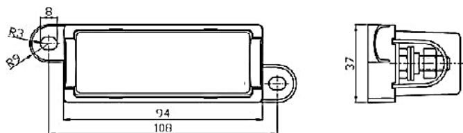
Fuse holder for MEGA fuse
